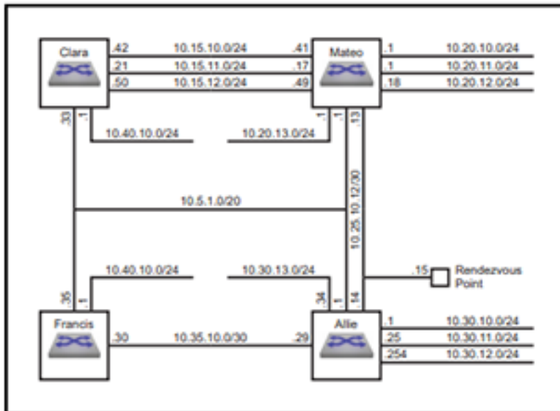
Figure 49: Multicast Example
