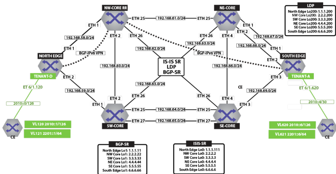
Figure 111: IPv6 VPN Physical Topology
