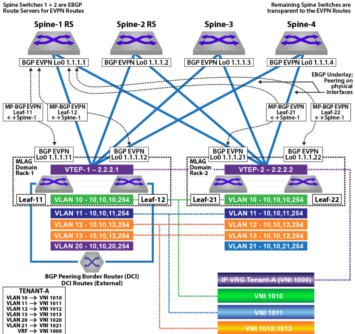
Figure 98: Tenant-A: Symmetric IRB
