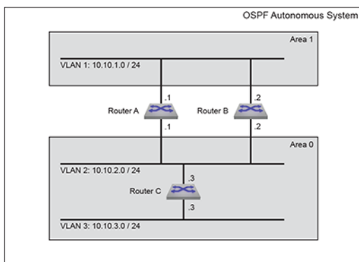
Figure 33: OSPFv2 Example 1
